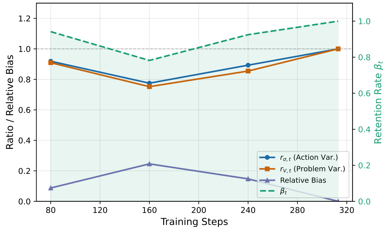
Qwen2.5-Math-1.5B (Oracle)
